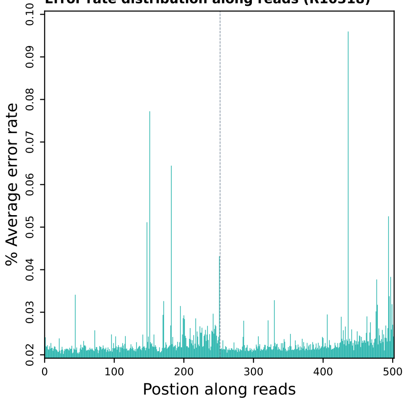
Error rate distribution along reads (R10318)
